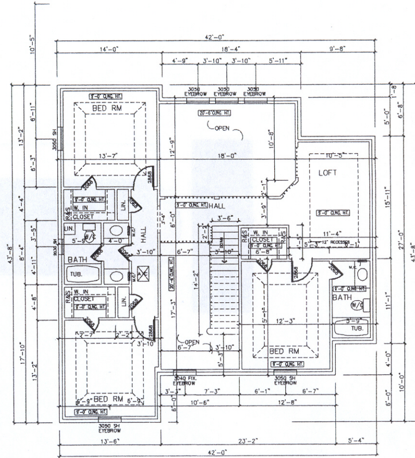
2 SECOND FLOOR PLAN SCALE: 1/4" = 1'-0"
