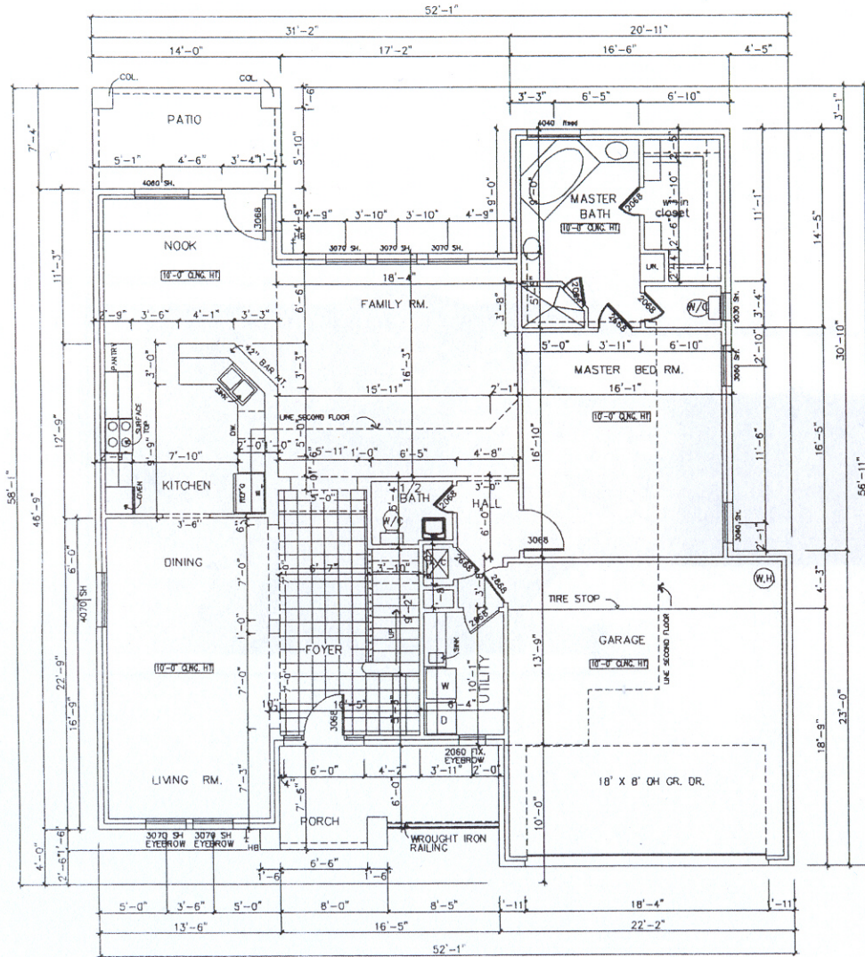
1 FIRST FLOOR PLAN SCALE: 1/4" = 1'-0"
